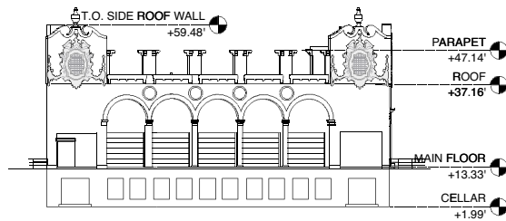
EXISTING ELEVATION BOARDWALK
