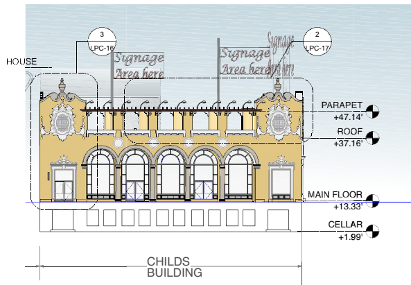
PROPOSED ELEVATION BOARDWALK
