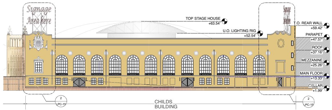
PROPOSED ELEVATION WEST 21ST STREET
